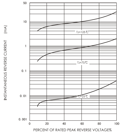
FIG.4-TYPICAL REVERSE CHARACTERISTICS
